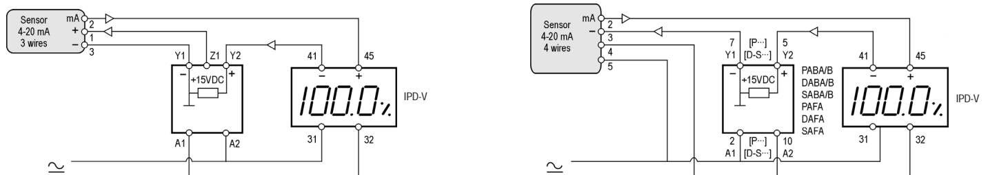
Visualization, supply of the sensor (3 wires) and 1 or 2 set points.
